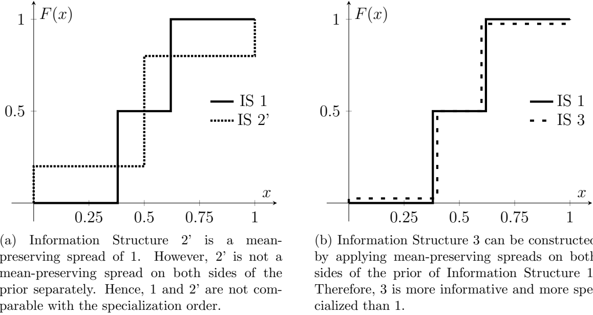
Figure 2: Illustration of specialization. Distribution of virtual posteriors.
